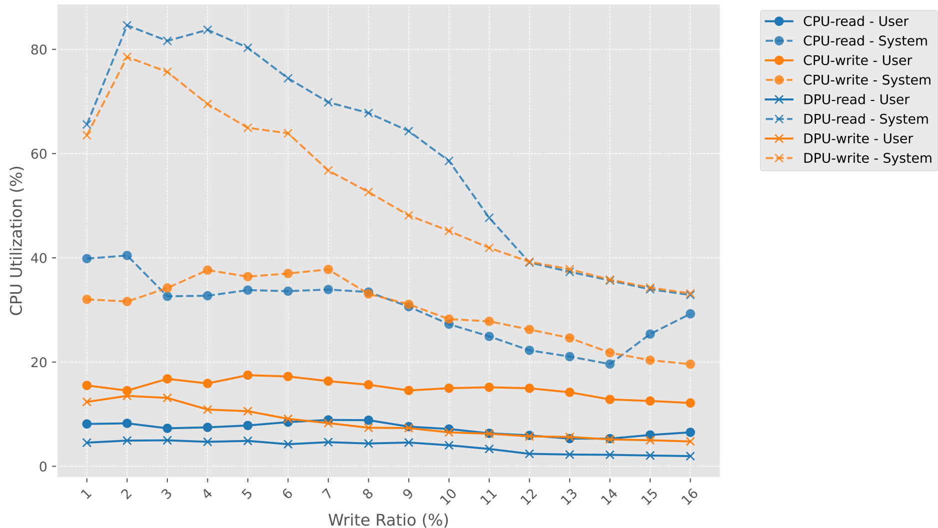
CPU Utilization vs Write Ratio (numjobs-bw)
